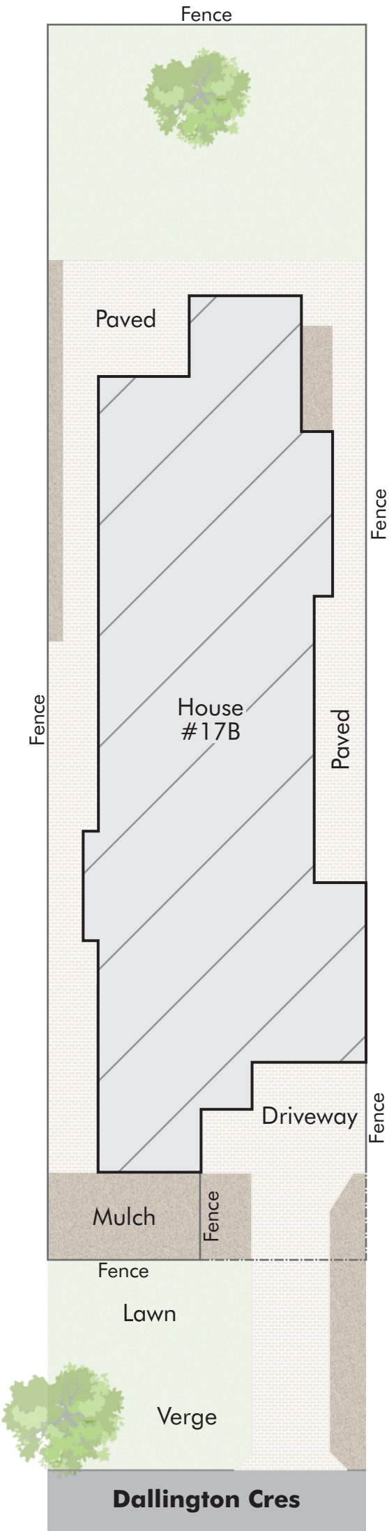
Site Plan
