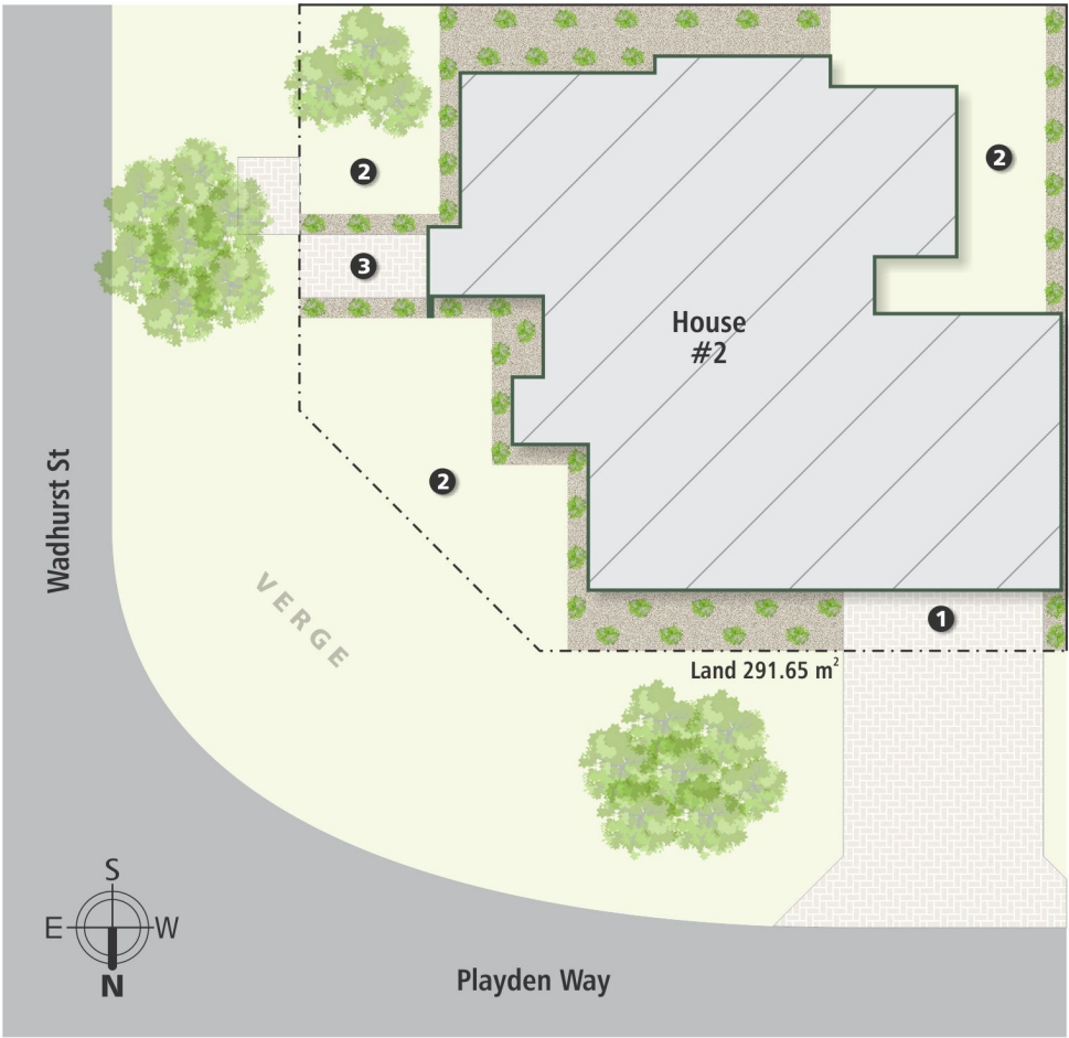
Site Plan
