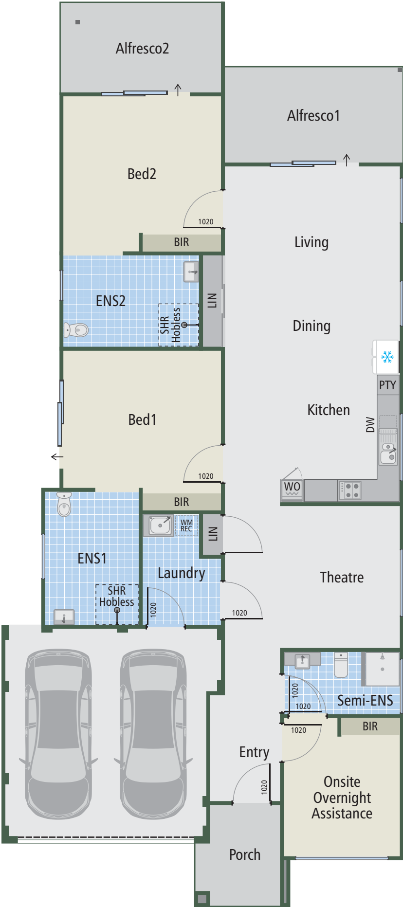
Floor Plan
